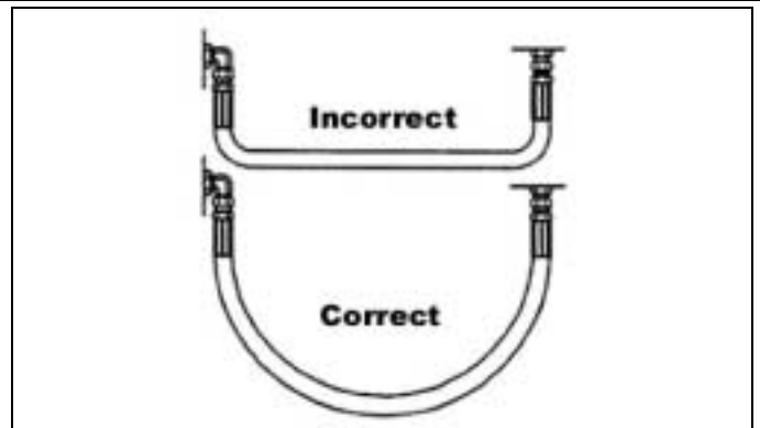
Fig.R7 Hose manufacturers minimum bend radius recommendations should be observed for both static connections and for connections to moveable mechanisms. Bend radius for connections with moveable mechanisms should be checked over the entire range of motion to prevent damage to the hose/tube assembly or connectors.
