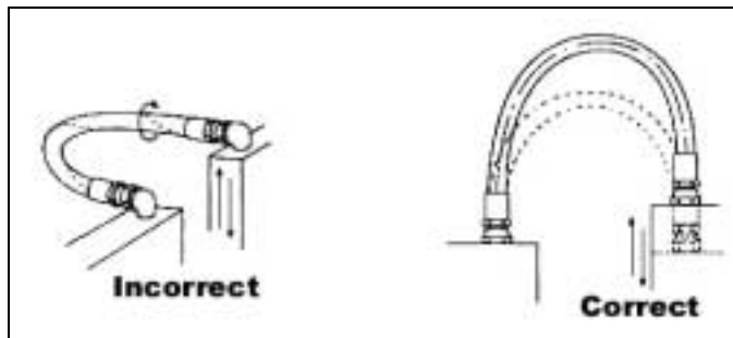
Fig.R11 When routing hose assemblies between components that move in a single plane relative to each other, provide connections that result in movement of the hose in the same plane of motion without twisting. Evaluate the total range of motion of the hose assembly to ensure that the minimum bend radius is not violated. Twisting of the hose will result in reduced pressure capability and can cause loosening of the fitting when the hose is pressurized. Bending the hose tighter than the minimum bend radius can exert excessive force on the connections and will reduce the hose service life.
