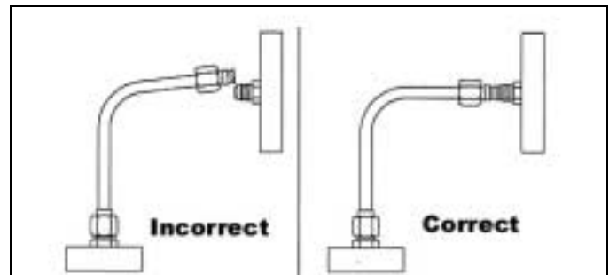
Fig.R1 Check for proper component alignment. Correct misalignment prior to final assembly. Align hose/tube assembly allowing hand connection. To assure proper alignment, two to three turns of nut should be easily permitted by hand.
