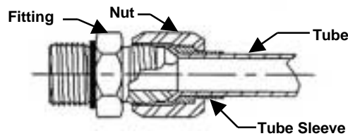
Fig.A1 37° Tube Fitting Assembly
